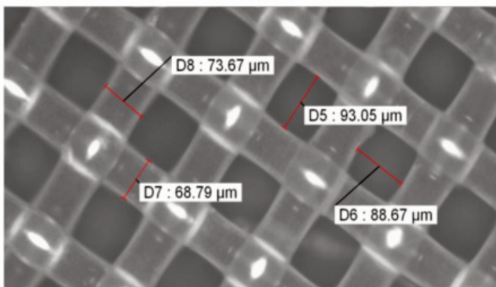
Sprint Filter - SF P08 (1 layer)
