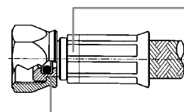
Connessione a doppia tenuta brevettata/ Connection with patented double seal
